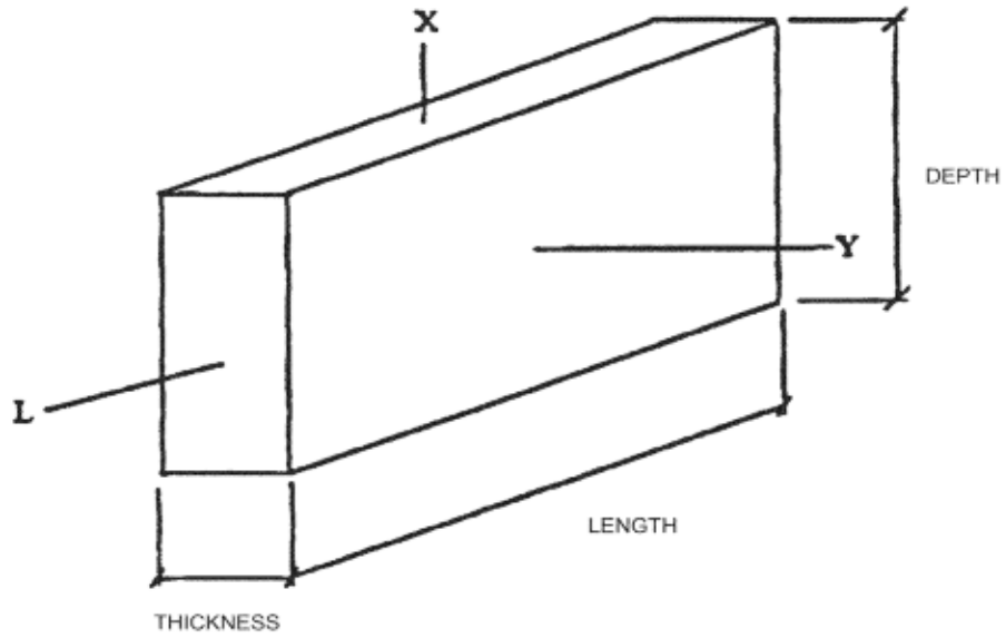
FIGURE 1—RIMBOARD ORIENTATION
