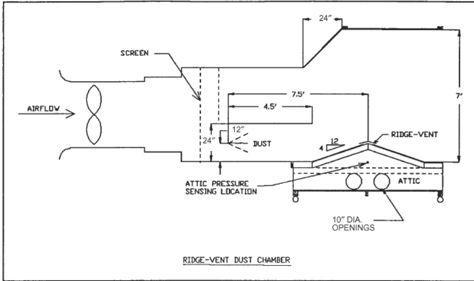
FIGURE 1—DUST-EXPOSURE TEST ON RIDGE VENTS
