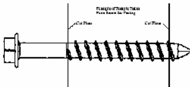
FIGURE 8.9—ILLUSTRATION OF TEST SPECIMEN EXTRACTION
