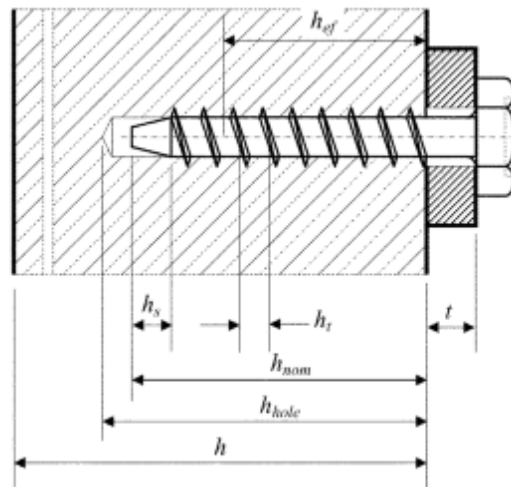
Fig. 2.6 – Effective embedment depth of screw anchors.
