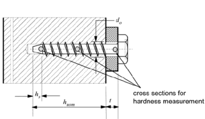
FIGURE 8.4—CONCRETE SCREW WITH SECTIONS FOR HARDNESS MEASUREMENT
