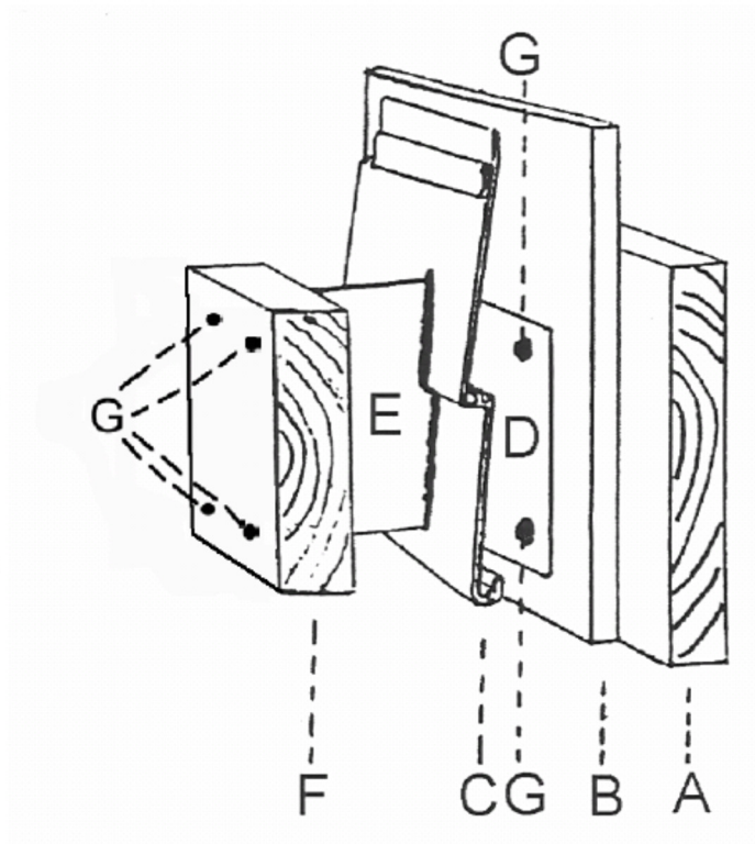
FIGURE 2—INSTALLATION DETAIL
