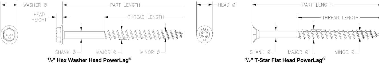
FIGURE 1D—1/2-INCH POWERLAG® SCREWS
