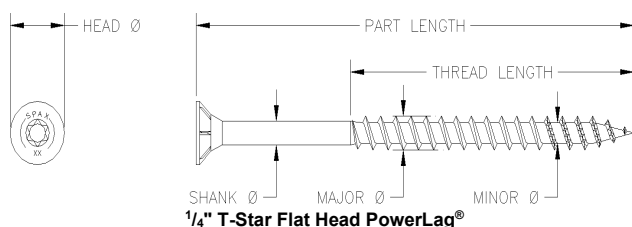
FIGURE 1A—1/4 INCH POWERLAG® SCREWS
