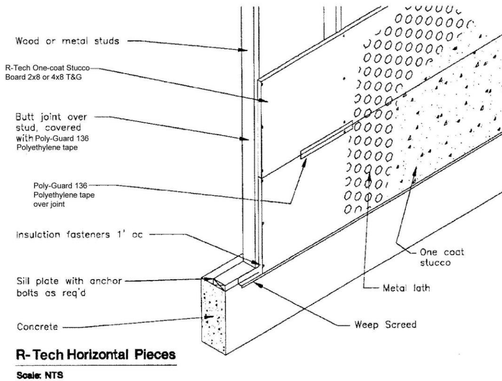
FIGURE 3—INSTALLATION DETAILS FOR R-TECH ONE-COAT STUCCO BOARD INSULATION USED AS A WEATHER-RESISTIVE BARRIER (Continued)
