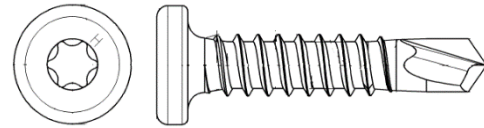
FIGURE 8—TORX PANCAKE HEAD (TPCH) SD FRAMER SELF-DRILLING SCREW
