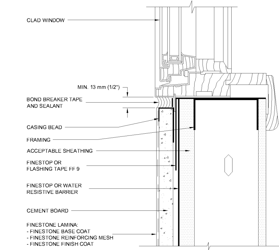
FIGURE 6—TYPICAL CLAD WINDOW SILL DETAIL
