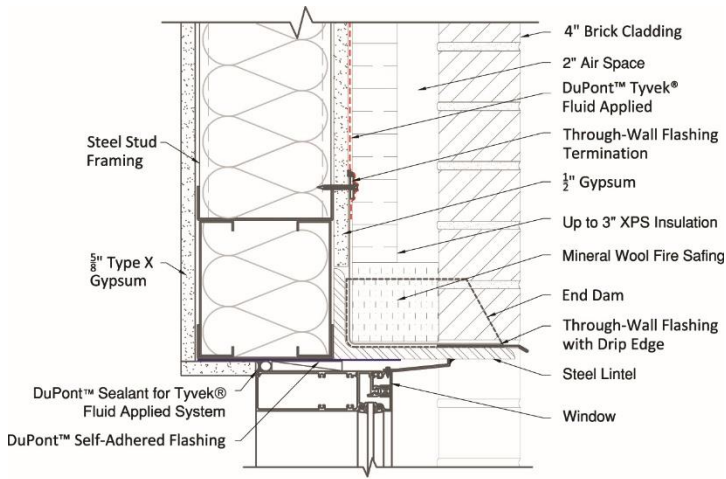
NFPA 285 Window Head Detail Option #1
