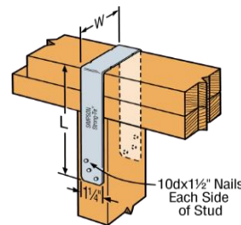
Typical SP4 Installation: Double Top Plate to Stud (SPH Similar)
