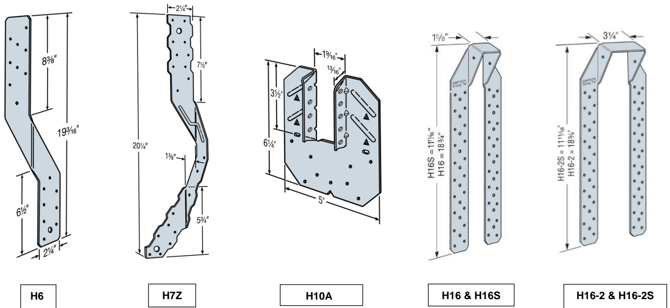
FIGURE 1b— H6, H7Z, H10A, H16, H16S, H16-2 AND H16-2S HURRICANE TIES
