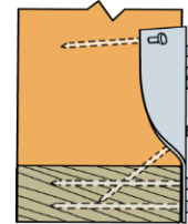
SP1 Nailing Profile
