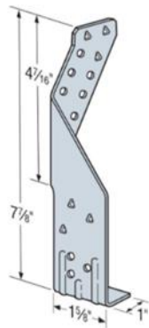
TSP U.S. Patent D618,085
