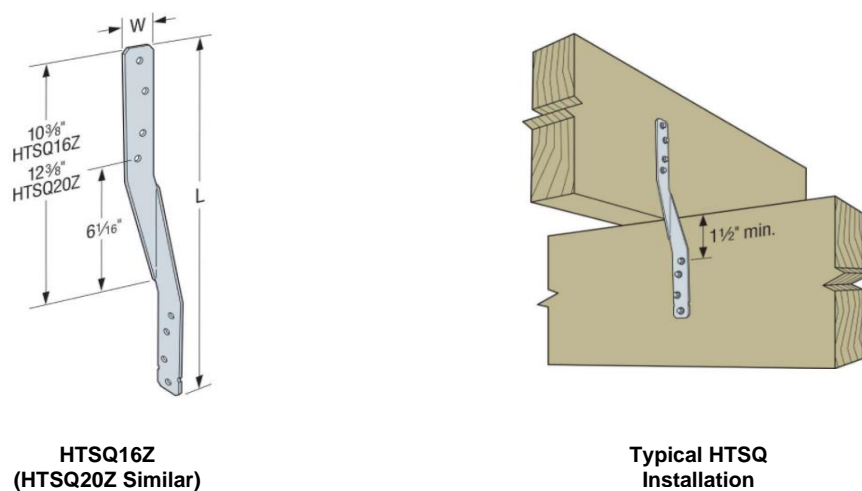
FIGURE 4—HTSQ TWIST STRAPS
