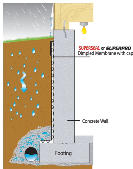
FIGURE 1—TYPICAL MEMBRANE INSTALLATION DETAIL
