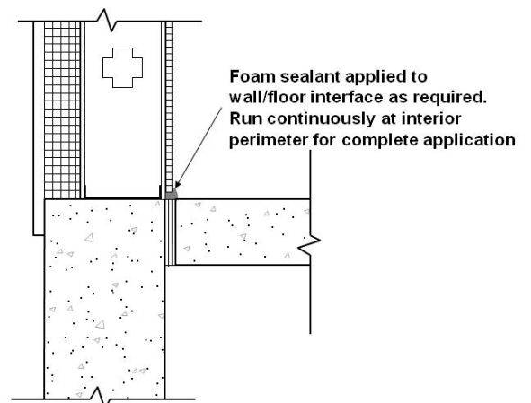
FIGURE 3—WALL/FLOOR JUNCTURE
