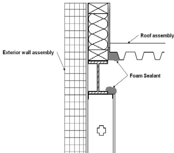
FIGURE 2—ROOF/WALL JUNCTURE
