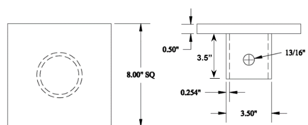
NCCH2788812 Bracket (for 2 7 / 8 x0.217-inch and 2 7 / 8 x0.203-inch Piles) Steel of plate conforms to ASTM A36 or ASTM A572 Gr. 50. Steel of tube conforms to API-5CT N80.
