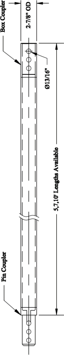
HELICAL EXTENSION SHAFT SECTION
