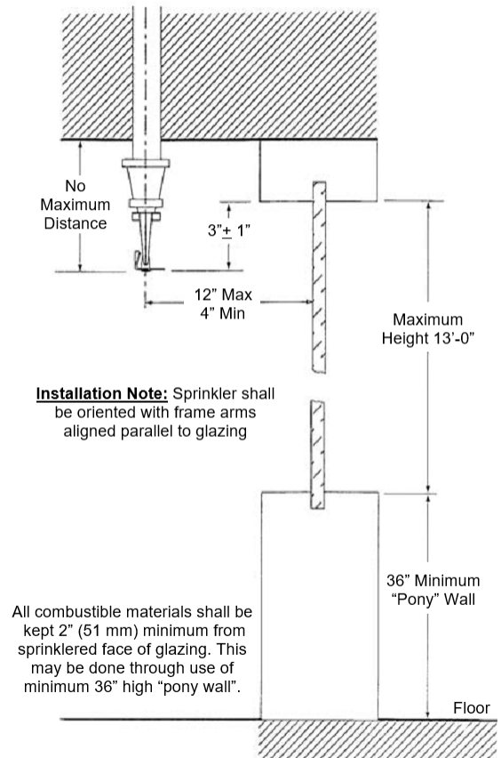
FIGURE 5—WS™ PENDENT VERTICAL SIDEWALL SPRINKLER INSTALLATION
