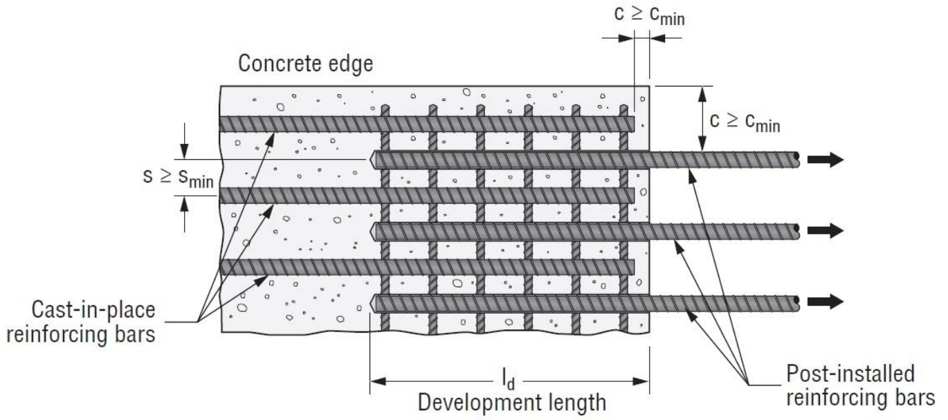
FIGURE 1—INSTALLATION PARAMETERS FOR POST-INSTALLED REINFORCING BAR CONNECTIONS
