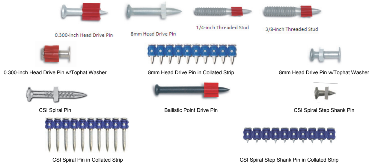
FIGURE 3—POWER-DRIVEN FASTENERS
