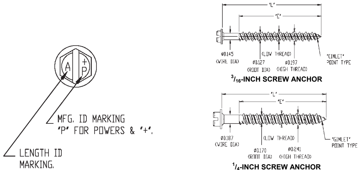
FIGURE 1—FASTENER SPECIFICATIONS FOR TAPPER+ SCREW ANCHOR (Slotted Hex Head Shown)
