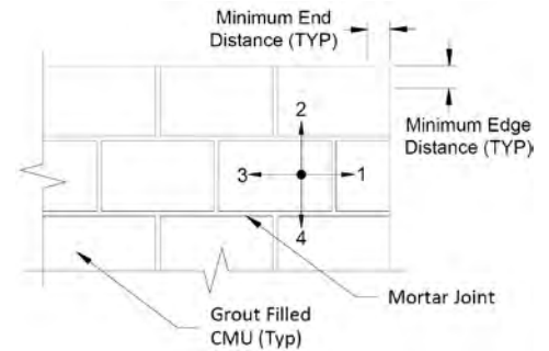
FIGURE 2—AC100+ GOLD ADHESIVE ANCHORS INSTALLED INTO THE TOP OF GROUTED CONCRETE MASONRY
