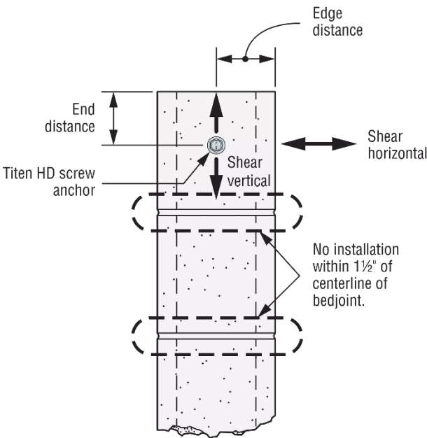
FIGURE 6—EDGE AND END DISTANCES FOR THE CARBON STEEL TITEN HD ANCHOR INSTALLED IN THE END OF HOLLOW CMU MANSORY WALL CONSTRUCTION (Refer to Table 9 )
