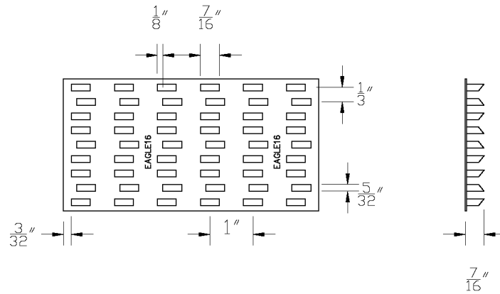
FIGURE 3 - EAGLE16 CONNECTOR PLATE
