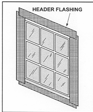
FIGURE 1—TYPICAL WINDOW FLASHING INSTALLATION
