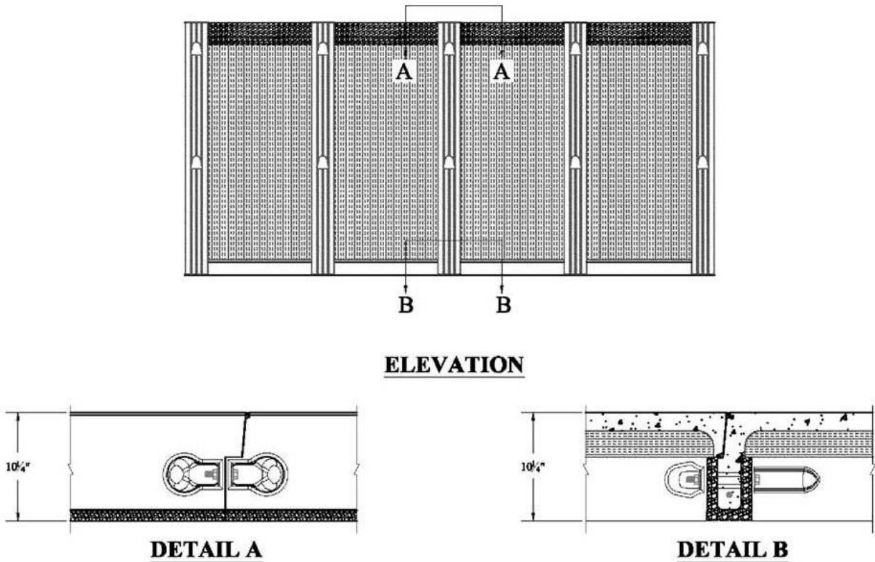
FIGURE 4—TYPICAL WALL CONNECTION
