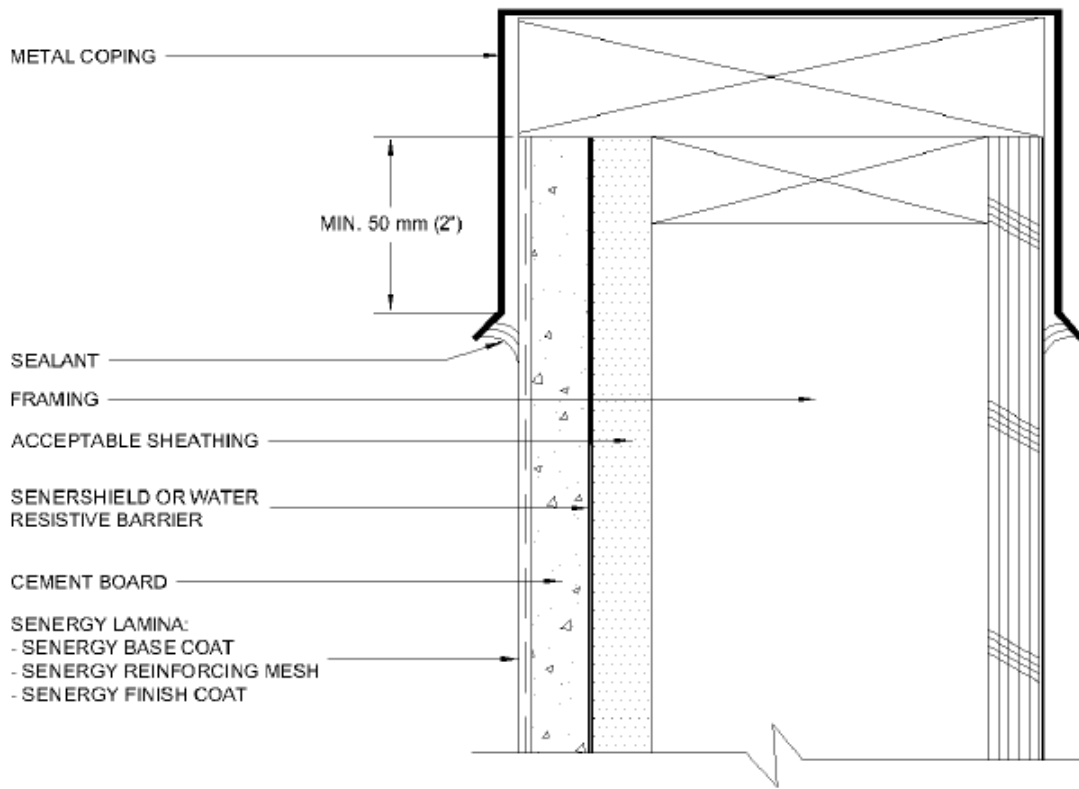
FIGURE 9—TYPICAL METAL COPING DETAIL
