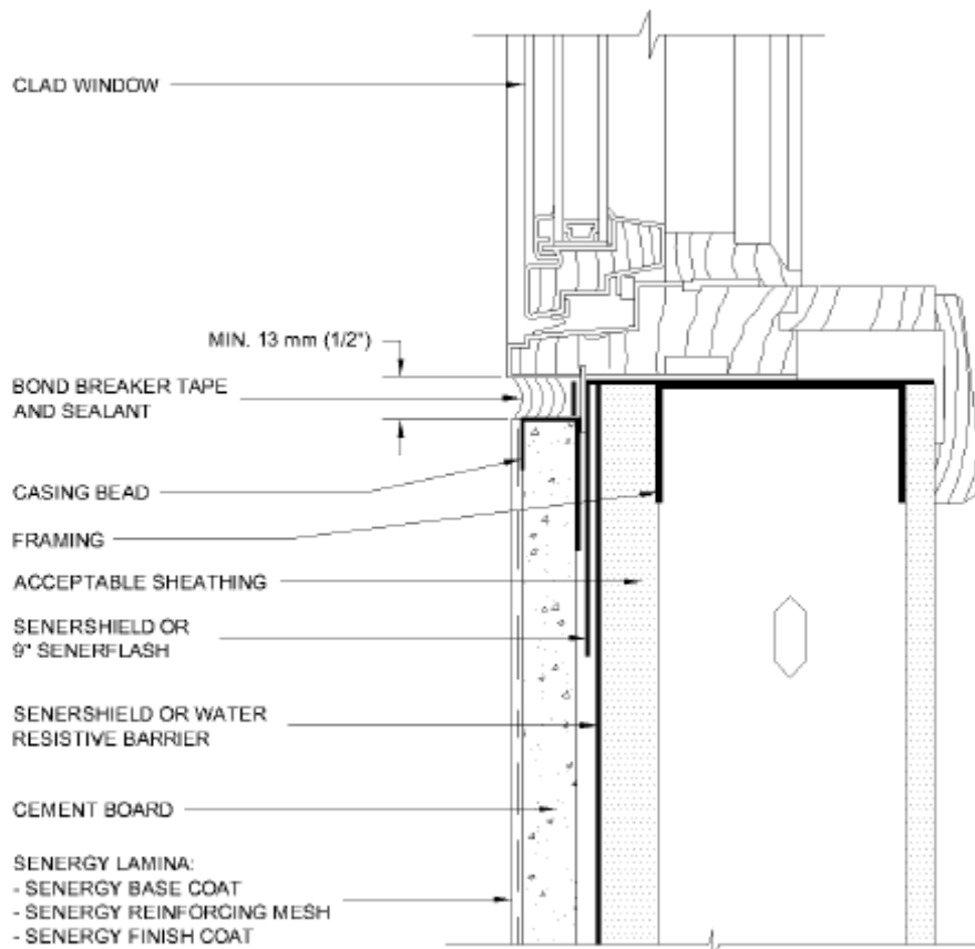
FIGURE 6—TYPICAL CLAD WINDOW SILL DETAIL
