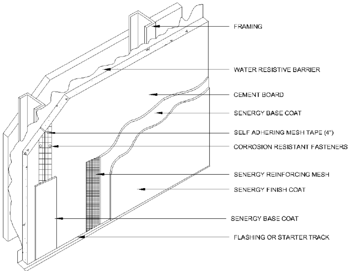
FIGURE 2—TYPICAL CEMENT-BOARD STUCCO SYSTEM 500 DESIGN (ISOMETRIC VIEW)
