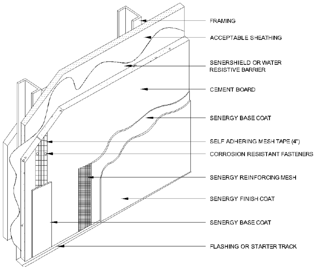
FIGURE 4—TYPICAL CEMENT BOARD STUCCO SYSTEM 1000 DESIGN (ISOMETRIC VIEW)
