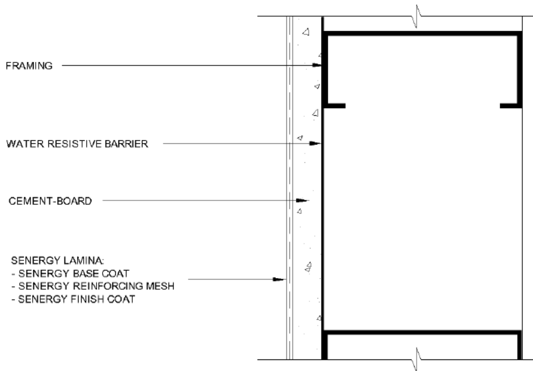
FIGURE 1—TYPICAL CEMENT BOARD STUCCO SYSTEM 500 DESIGN APPLICATION (PLAN VIEW)
