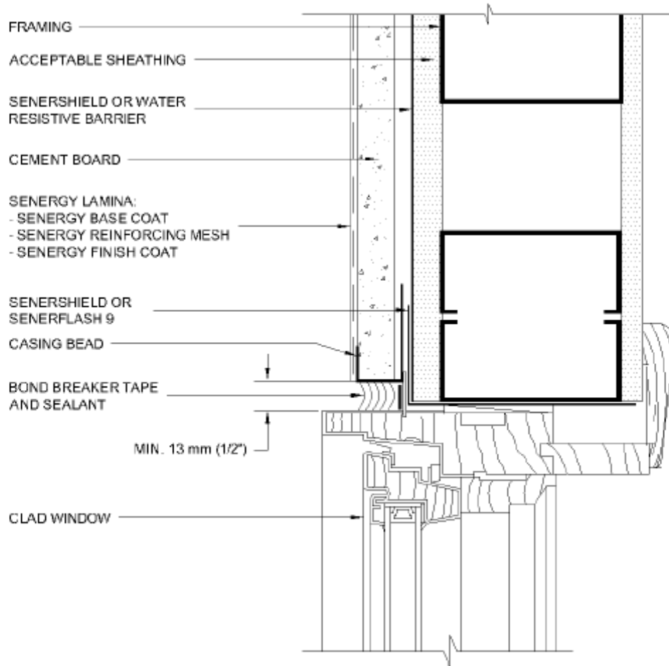
FIGURE 5—TYPICAL CLAD WINDOW JAMB DETAIL
