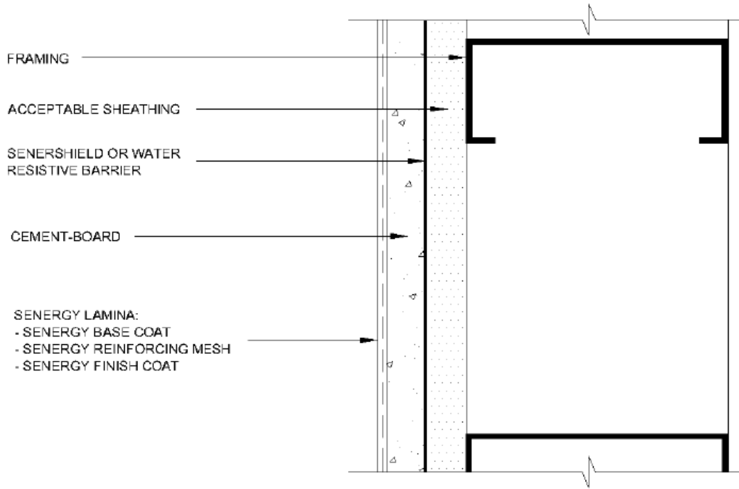
FIGURE 3—TYPICAL CEMENT-BOARD STUCCO 1000 SYSTEM DESIGN APPLICATION (PLAN VIEW)
