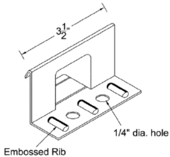
FIGURE 4—SL-1750 ANCHOR CLIP For SI: 1 inch = 25.4 mm
