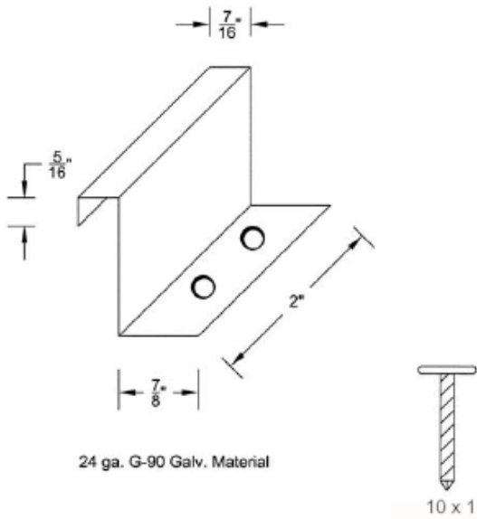
FIGURE 2—CB-150 ANCHOR CLIP For SI: 1 inch = 25.4 mm
