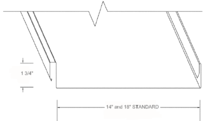
FIGURE 3—SL-1750 PANEL For SI: 1 inch = 25.4 mm
