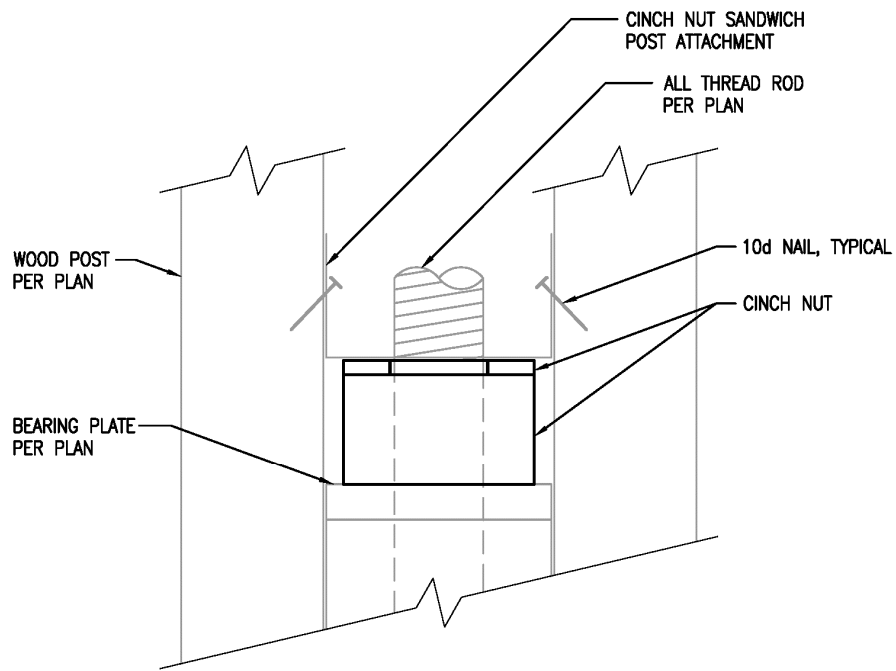
FIGURE 2—CINCH NUT INSTALLATION DETAIL—SANDWICH POST SYSTEM
