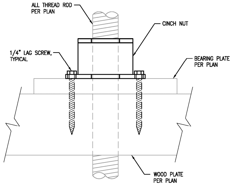
FIGURE 3—CINCH NUT INSTALLATION DETAIL—PLATED SYSTEM
