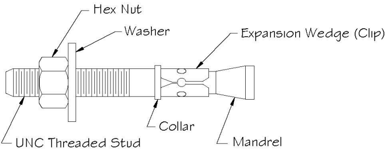
FIGURE 1—POWER BULL WEDGE ANCHOR
