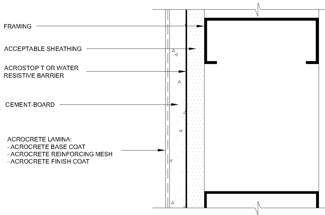
FIGURE 3—TYPICAL ACROWALL-CBS DESIGN APPLICATION (PLAN VIEW)
