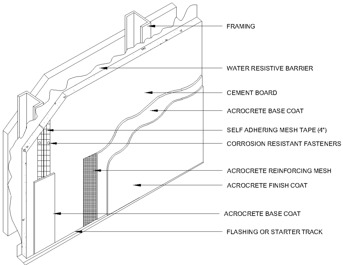
FIGURE 2—TYPICAL ACROWALL-CBS 500 DESIGN (ISOMETRIC VIEW)
