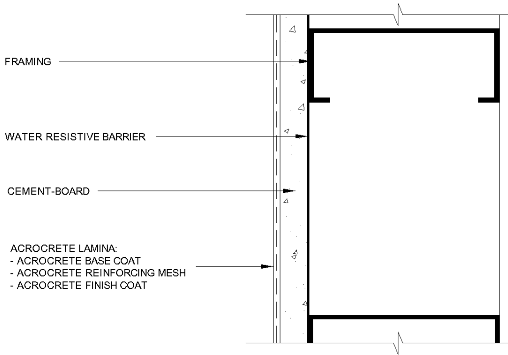
FIGURE 1—TYPICAL ACROWALL-CBS 500 DESIGN APPLICATION (PLAN VIEW)
