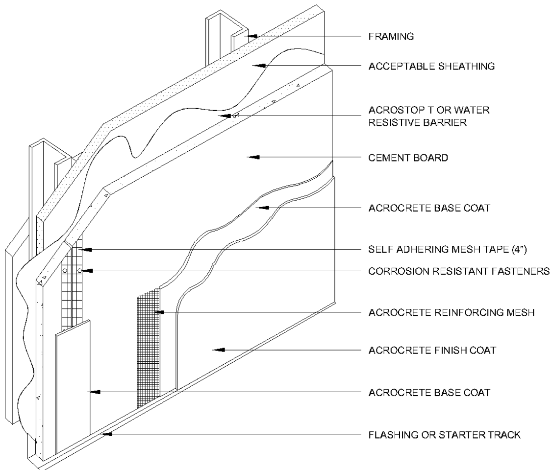
FIGURE 4—TYPICAL ACROWALL-CBS DESIGN (ISOMETRIC VIEW)
