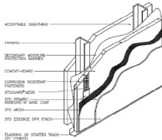
TYPICAL STOQUIK SILVER I CEMENT-BOARD STUCCO SYSTEM
