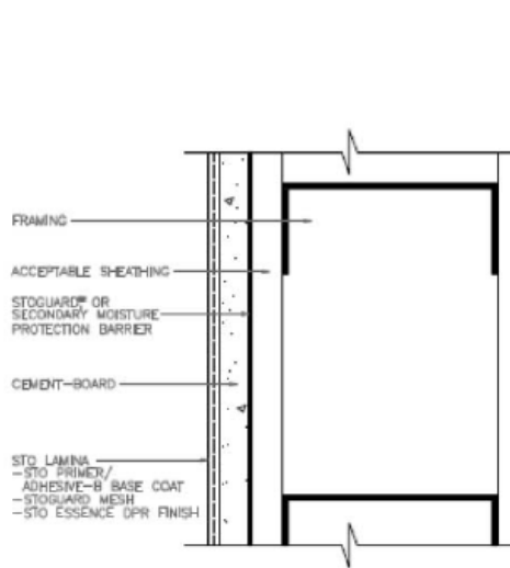
TYPICAL STOQUIK SILVER II CEMENT-BOARD STUCCO SYSTEM DESIGN APPLICATION (PLAN VIEW)
