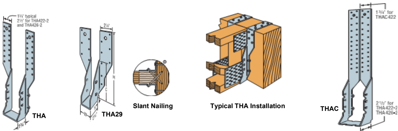
FIGURE 4—THA SERIES TRUSS HANGERS ADJUSTABLE
