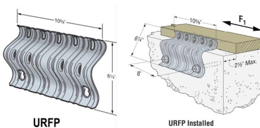
FIGURE 7—URFP UNIVERSAL RETROFIT FOUNDATION PLATE
