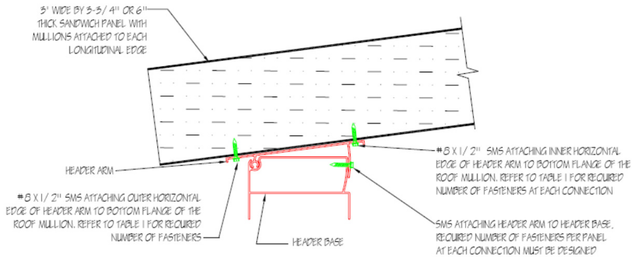
FIGURE 2—HEADER TO ROOF SYSTEM CONNECTION DETAIL
