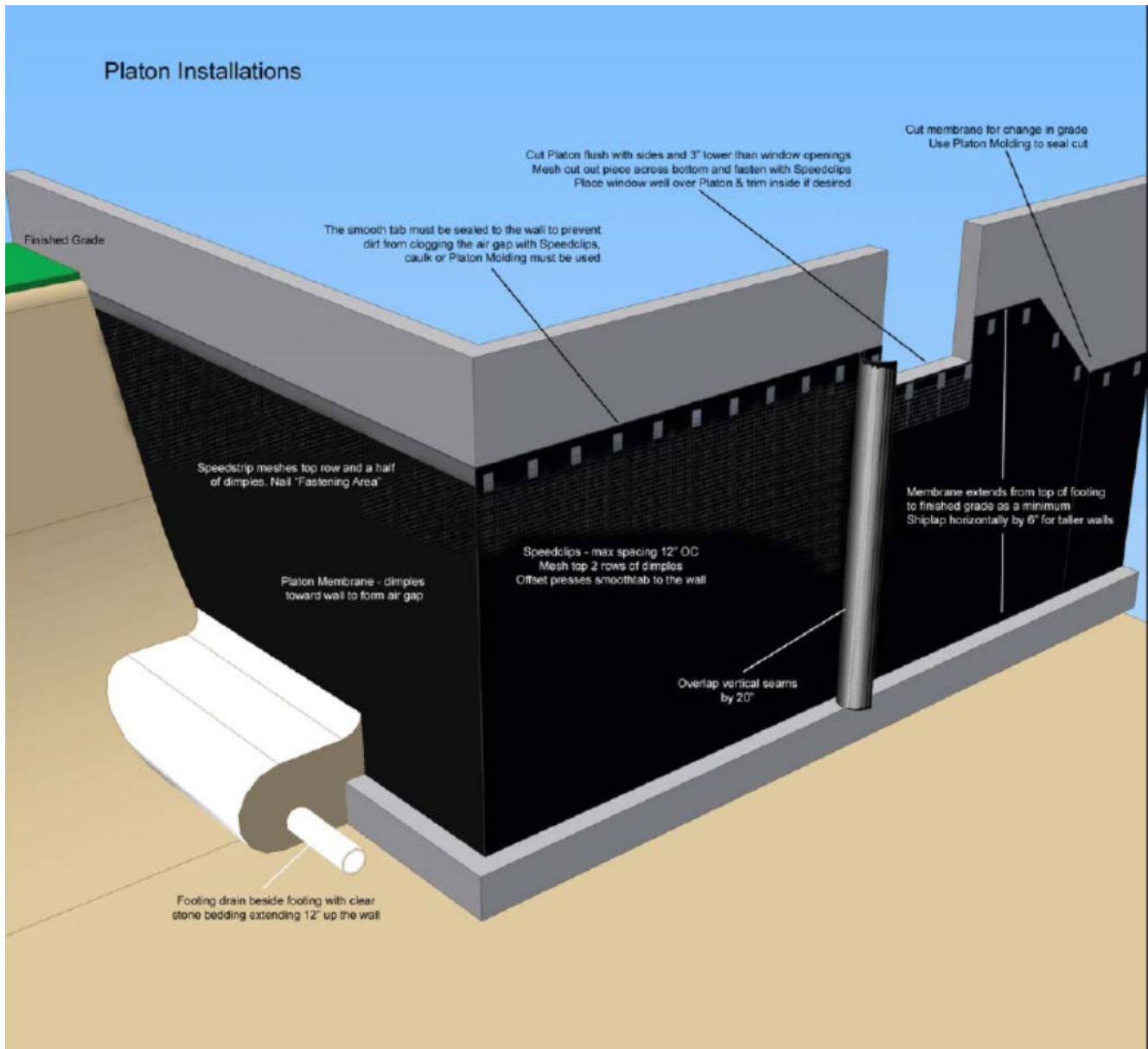
FIGURE 2—INSTALLATION DETAILS
