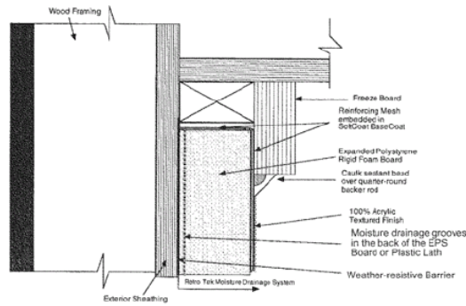
Typical Moisture Drainage Soffit Termination
