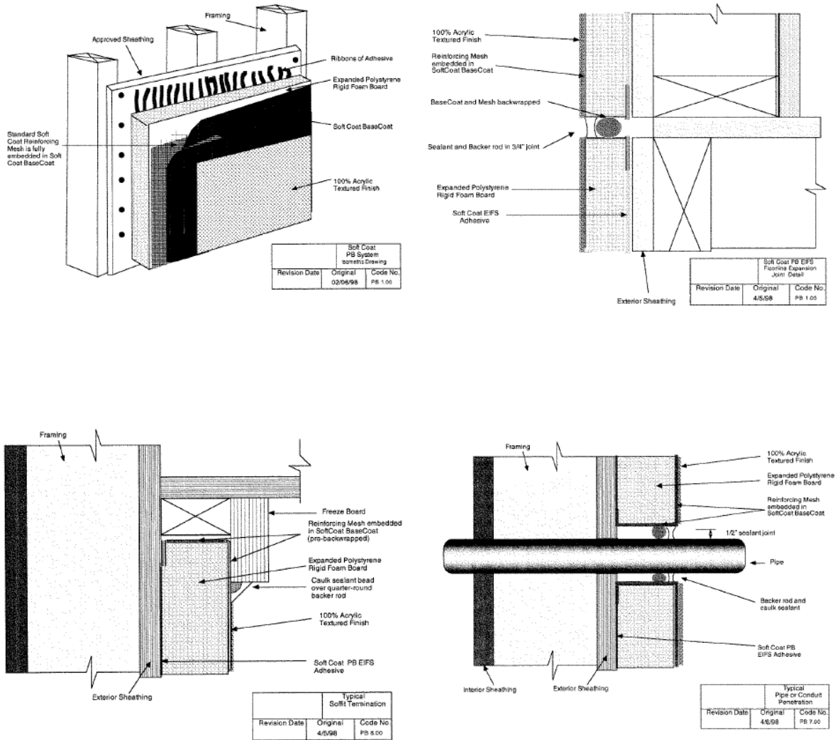
FIGURE 4—SOFTCOAT PB SYSTEM—TYPICAL DETAILS
