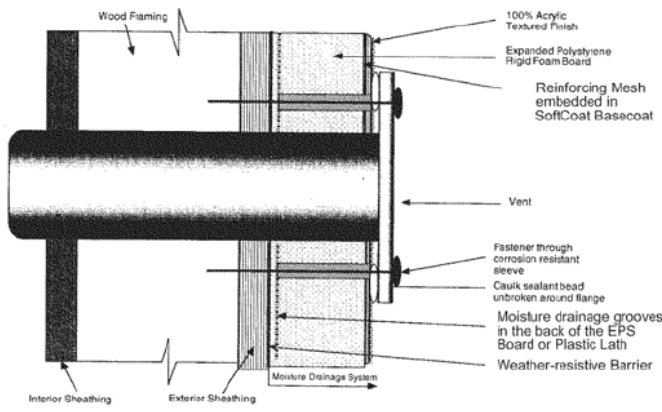
Typical Vent Detail
