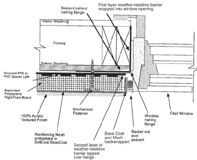
Typical Moisture Drainage Window Jamb Detail
