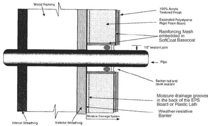
Typical Pipe or Conduit Penetration
