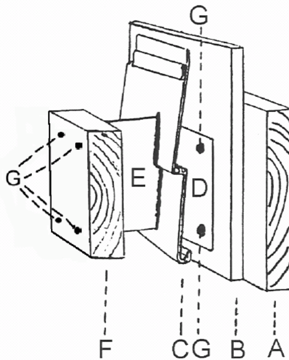
FIGURE 2—INSTALLATION DETAIL
