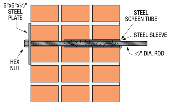
FIGURE 1—ANCHOR INSTALLATIONS FOR UNREINFORCED BRICK MASONRY (Refer to Sections 4.1 through 4.3 for details concerning design and installation of anchors in unreinforced brick masonry)
