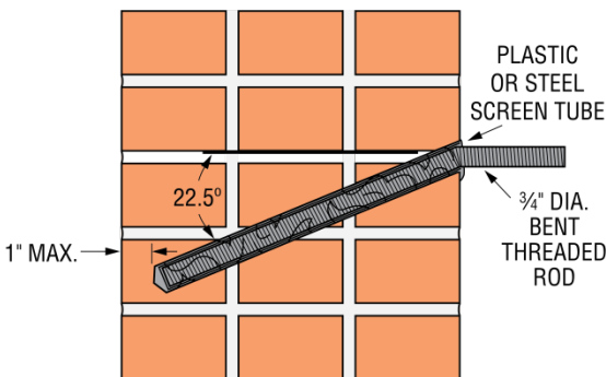
FIGURE 1—ANCHOR INSTALLATIONS FOR UNREINFORCED BRICK MASONRY (Refer to Sections 4.1 through 4.3 for details concerning design and installation of anchors in unreinforced brick masonry)
