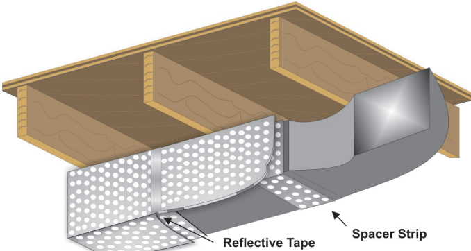
Big-8 Spacer Wrap for an R-8 Value (With Spacer Strips)
