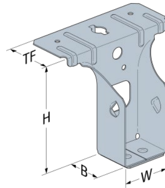
FIGURE 4b—PF24B HANGER
