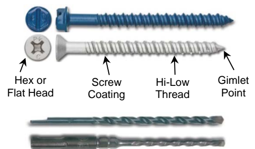
FIGURE 2—ULTRACON+ SCREW ANCHORS AND DRILL BITS (slotted hex head and flat head versions pictured)
