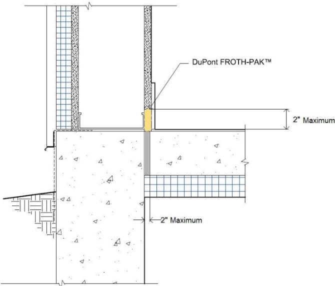
FIGURE 3—EXAMPLE OF WALL/FLOOR JUNCTURE APPLICATION OF FOAM
